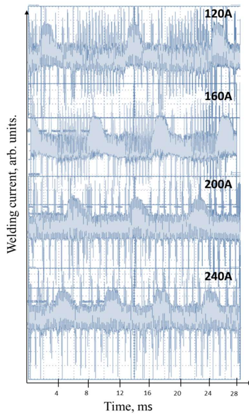
Fig. 5. Waveforms for inverter power supply, pulse welding mode (schematic view)
