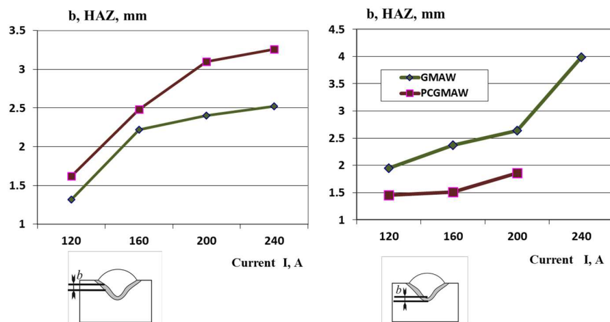
Fig. 7. Effect of the average welding current (during GMAW and PCGMAW) on the HAZ width (b, mm)
