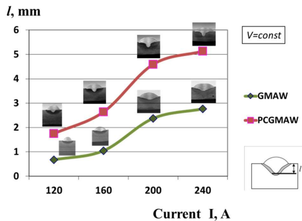
Fig. 8. Effect of the average welding current (during GMAW and PCGMAW) on the penetration depth ( l ) and on the shape of the seam. Welding speed V=\text{const}
