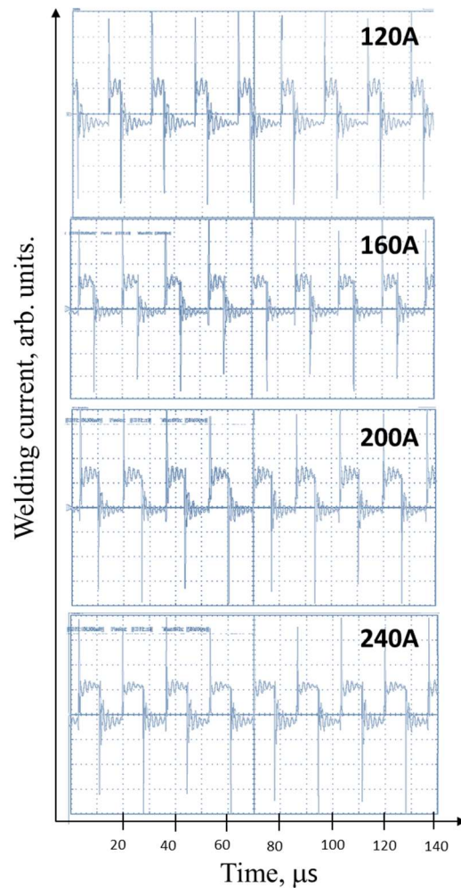
Fig. 2. Waveforms for inverter power supply, stationary welding mode
