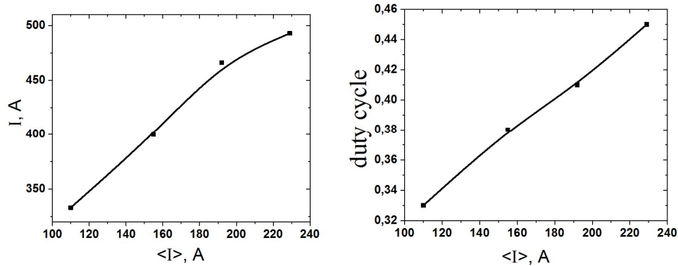
Fig. 3. Dependence of average welding current \langle I \rangle and momentum current I (a), duty cycle (b)
