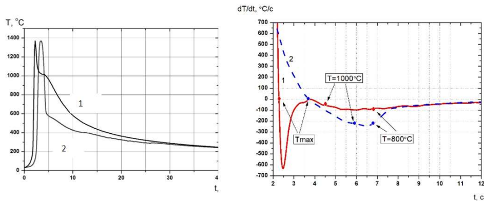
Fig. 6. Welding Thermal Cycles (a) and derivative of WTC (b) for PCGMAW (1) and GMAW (2)
