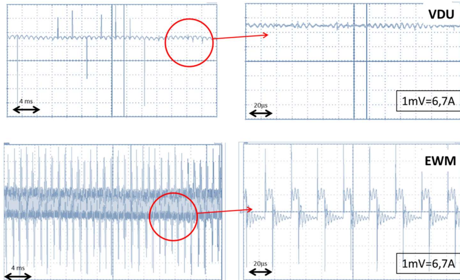
Fig. 1. Welding current waveforms for (a) transformer and (b) inverter types of power supplies (schematic view)
