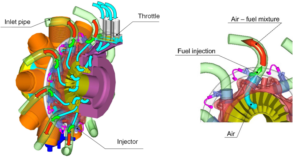
Fig. 2. The scheme of air and fuel flow in an intake system (ASz-62IR engine)
