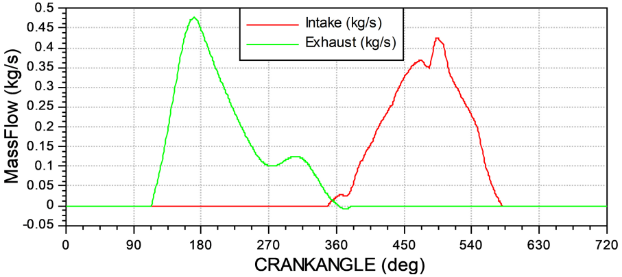
Fig. 9. Characteristics of mass flow [16]
