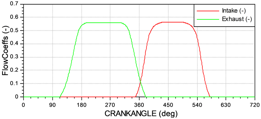
Fig. 8. Characteristics of valves flow coefficient [16]
