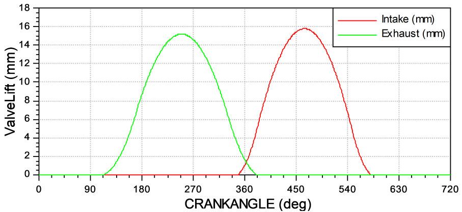
Fig. 5. Characteristics of valve lifts [16]
