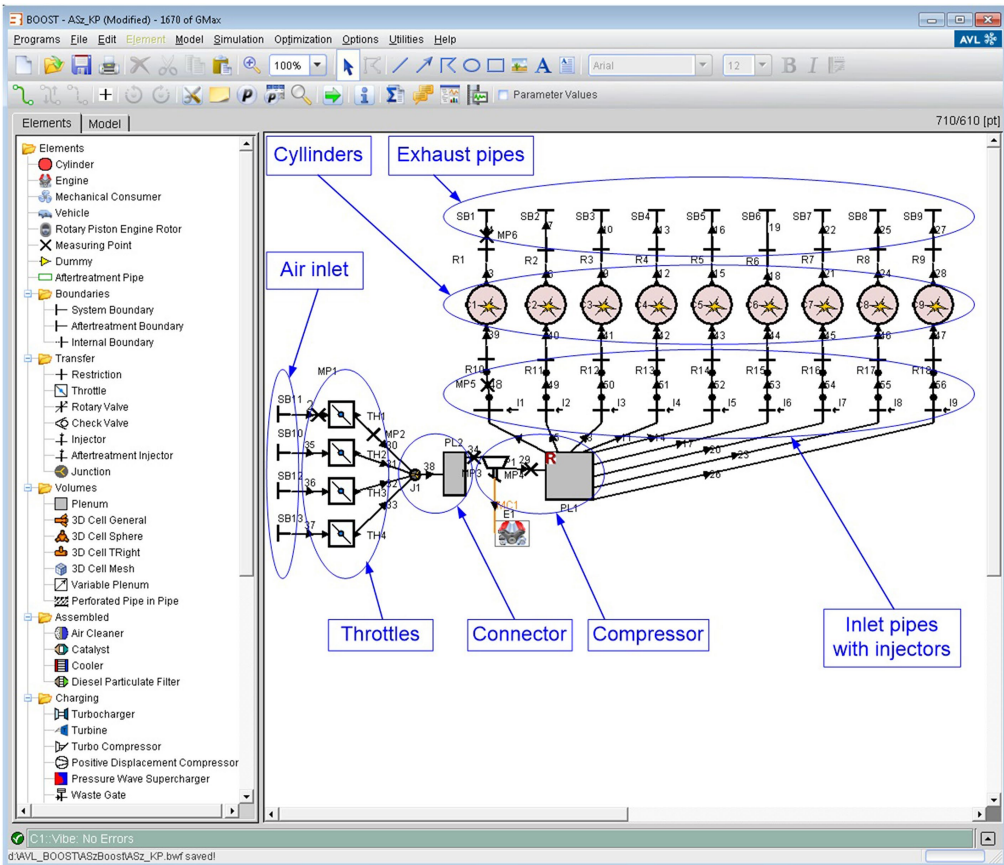
Fig. 3. AVL BOOST engine model [16]
