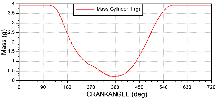
Fig. 10. Characteristics of air-fuel mixture mass in cylinder [16]
