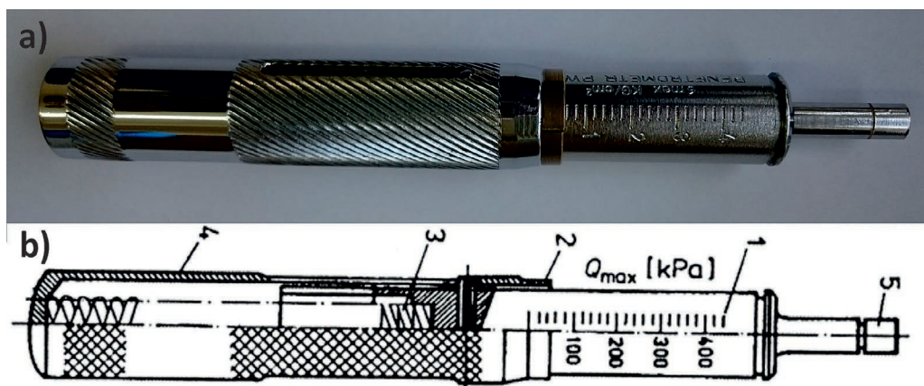
Figure 4. Pocket penetrometer: a) general view (photo by A. Gruchot), b) scheme [Myślińska 2006]: 1 – measurement scale, 2 – indicator ring, 3 – spring, 4 – handle, 5 – cylindrical tip of a diameter of 6.4 mm
