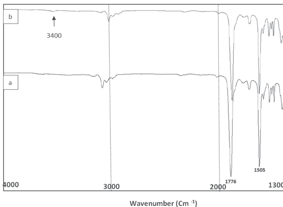
Fig. 4. The FTIR spectrum of polycarbonate film (A: control; B: treated with B. megaterium )
