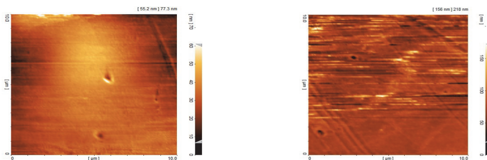
Fig. 3. AFM figures of surface erosion of polycarbonate films; A: Control; B: treated with B. megaterium ; cavities and bacterial biofilm are shown as dark and light areas on PC plastic surfaces, respectively
