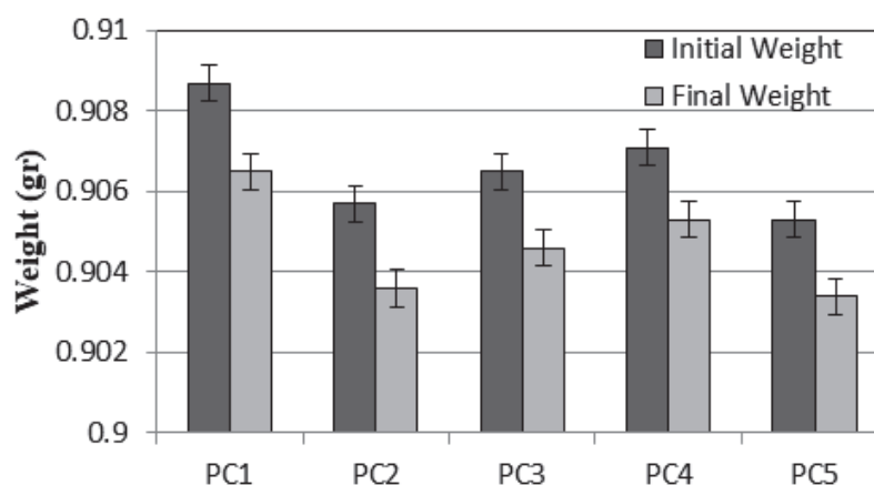
Fig. 1. The initial and final weight of PC films before and after 9 months burial (The error bars show the significant difference between initial and final weight of each PC films)
