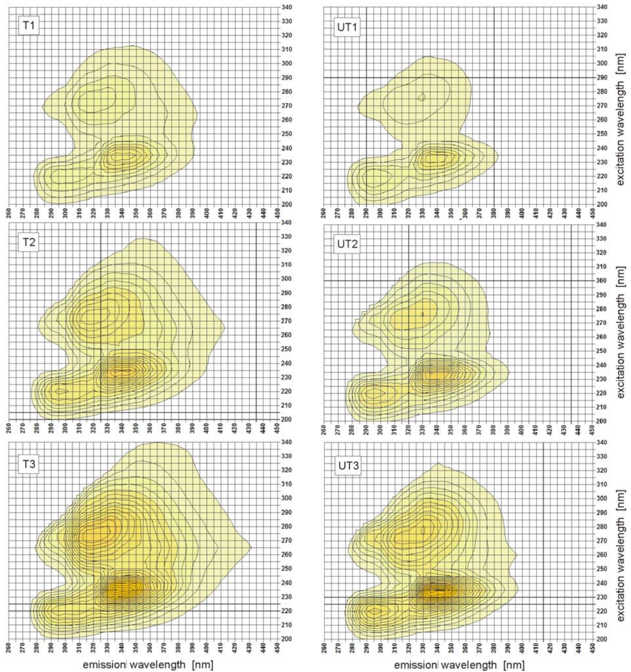
Fig. 3. Normalised excitation-emission fluorescence spectra as 2D map of oil in n-hexane dilutions for Titan Truck Plus 15W40 in tree oil concentrations T1, UT1: 25 mg/kg, T2, UT2: 50 mg/kg, T3, UT3: 100 mg/kg
