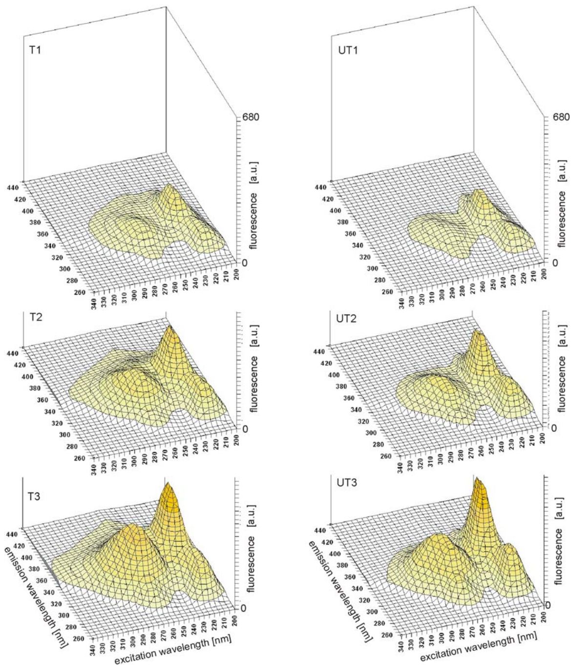
Fig. 2. Excitation-emission fluorescence spectra (EEMs) of oil in n-hexane dilutions in 3D plane for Titan Truck Plus 15W40 in three oil concentrations T1, UT1 : 25 mg/kg, T2, UT2 : 50 mg/kg, T3, UT3 : 100 mg/kg
