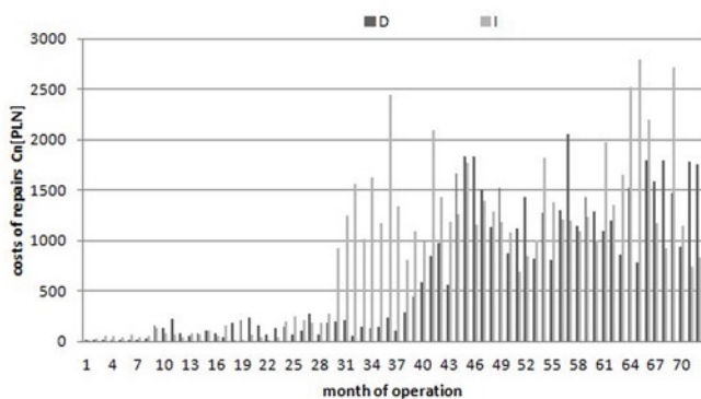
Fig. 3. Monthly costs of repairs per 1 bus [9]
