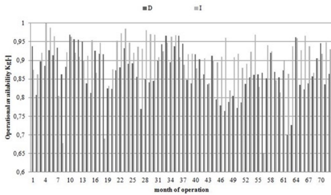
Fig. 1. Operational availability of buses as a function of time of operation on a monthly basis [12]
