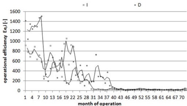
Fig. 4. The course of operational efficiency of buses as a function of time of operation on a monthly basis
