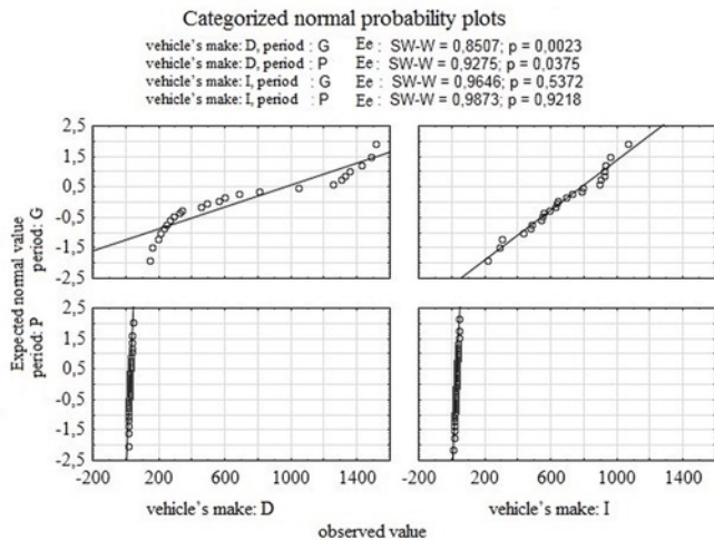
Fig. 5. Categorized diagrams of the normality of a dependent variable - operational efficiency of D and I buses during the warranty period (G) and post-warranty (P)
