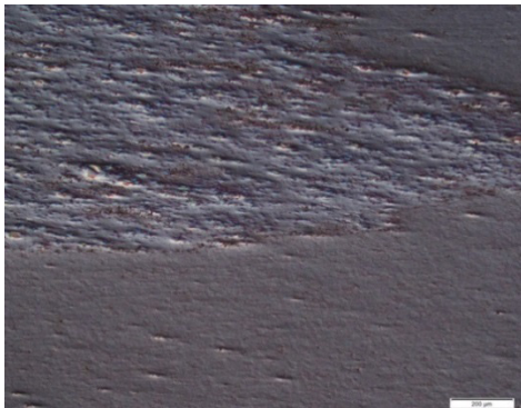
Fig. 10. Fragment of a structure from Fig. 6. EN AC-43200 alloy (from top) located on the advancing side after friction welding process (Nomarski contrast)
