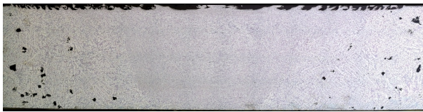
Fig. 16. Macrostructure of FSW weld (in the central zone) in the EN AC-43200
