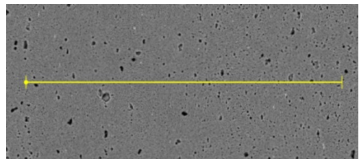
Fig. 14. Fragment of the structure from Fig. 8. Welding parameters: \omega = 900 \text{ min}^{-1} , V = 224 \text{ mm/min} . Triflute pin. SEM-EDS chemical composition analysis was conducted along the marked line (Fig. 15)
