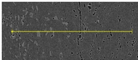
Fig. 12. Fragment of the structure from Fig. 6. The boundary between EN AC-43200 alloy (from the left side) and EN AW-6082 alloy (from the right side). Welding parameters: \omega = 450 \text{ min}^{-1} , V = 224 \text{ mm/min} . Triflute pin. SEM-EDS chemical composition analysis was conducted along the marked line (Fig. 13)
