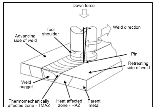
Fig. 1. The scheme of the FSW process [1]
