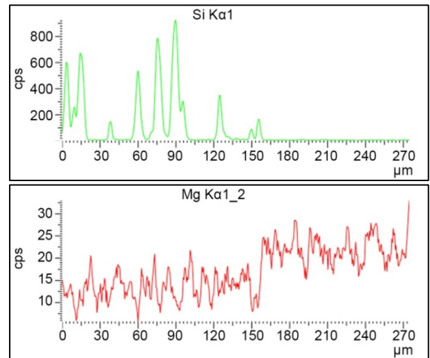
Fig. 13. Concentration of Si and Mg along the measuring line from Fig. 12
