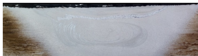
Fig. 9. Structure of FSW weld in the case of locating the rod of EN AC-43200 (A) on the retreating side. Welding parameters: \omega = 900 \text{ min}^{-1} , V = 224 \text{ mm/min} . Triflute pin. Etching: Keller
