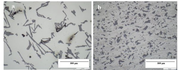
Fig. 18. Structures of casting alloy before FSW – a) and after FSW process – b) (SEM)
