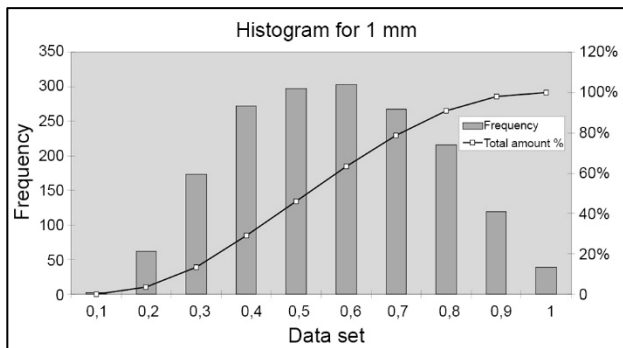
Fig. 17. Distribution of shape factor value basing on the data from EBSD [14]
