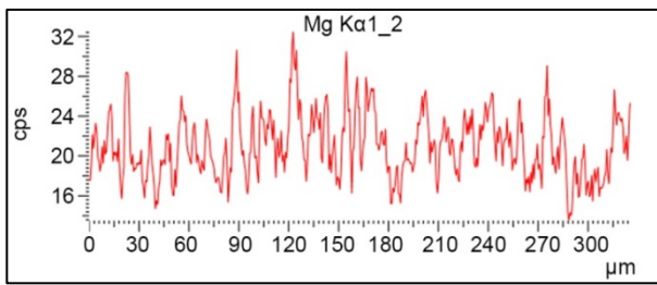
Fig. 15. Concentration of Si and Mg along the measuring line from Fig. 14
