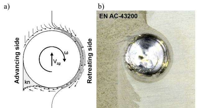
Fig. 4. Schematic image of the metal motion around the tool pin (a) and cross-section of the joint perpendicular to tool axis, in the place of retracted tool pin (b); kn – place of possible forming of wormhole discontinuities
