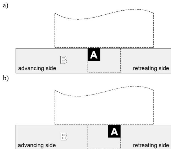
Fig. 5. Diagram of location of the rod of EN AC-43200 alloy (A) in the material of EN AW-6082 alloy (B) before welding with FSW process, a) from the advancing side; b) from the retreating side
