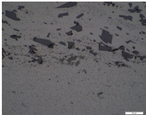
Fig. 11. Fragment of the structure from Fig. 6. Joining of EN AC-43200 metal layer (from top) with EN AW-6082 alloy
