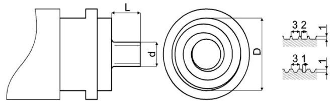
Fig. 3. Structure of a working part of FSW process tool
