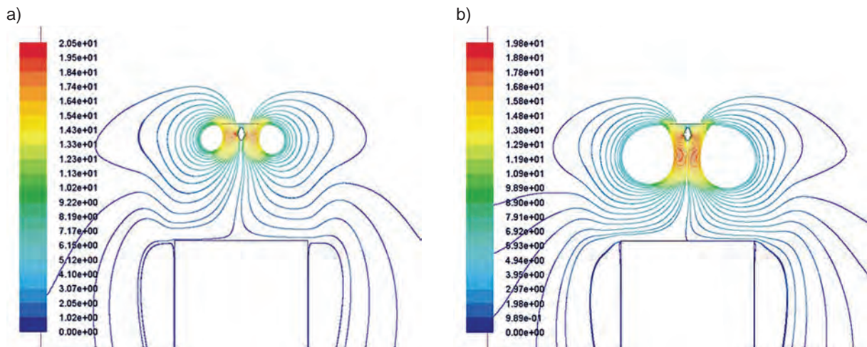
Fig. 1. Disturbances caused by helicopter in case of operating above building: a) hovering above building, b) approach for landing on a platform-disturbances of walls flow round view
