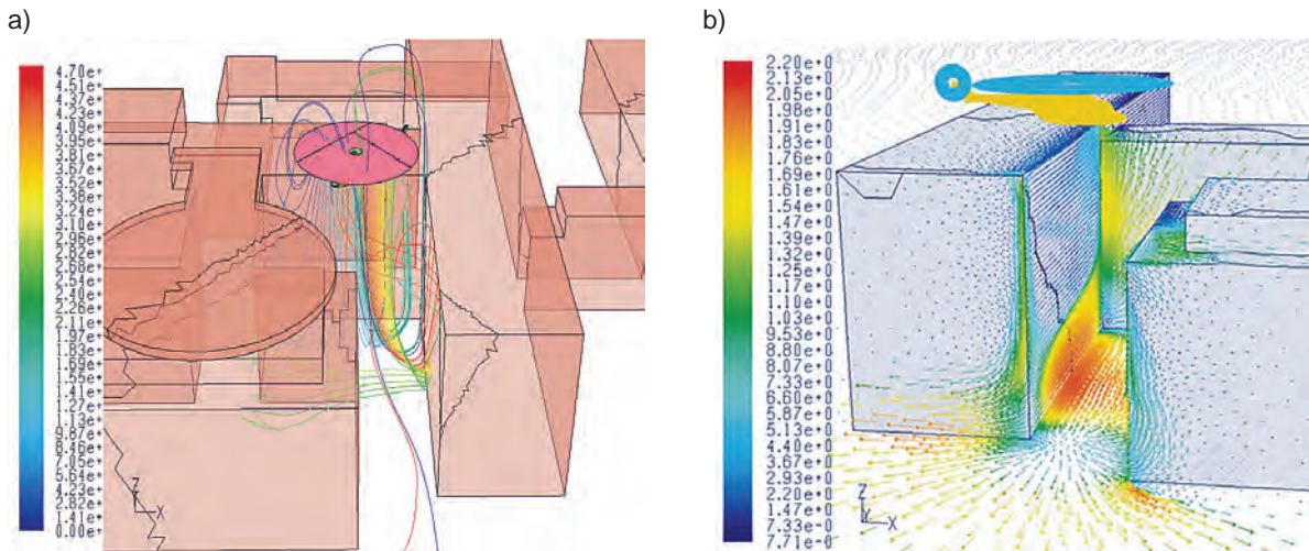
Fig. 3. Disturbances caused by helicopter during roof helipad operations: a) approach for landing on a platform, b) view of building walls flow round disturbances
