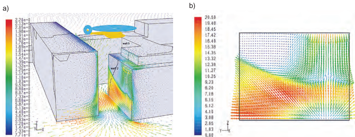
Fig. 2. Another view with walls designations and wall nr 2 flow round view
