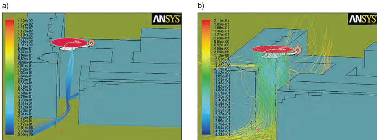
Fig. 4. Disturbances caused by helicopter during roof helipad operations: a) exhaust streams from engine nozzles, b) rotor stream lines flowing building around
