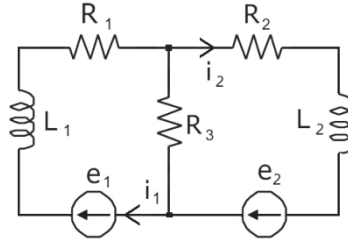
Fig.4.1. Positive electrical circuit
