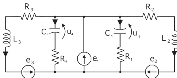
Fig. 4.3. Positive electrical circuit
