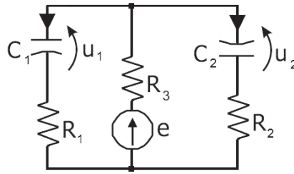
Fig.4.2. Positive fractional electrical circuit
