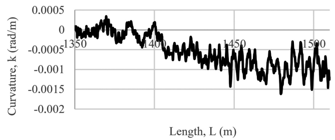
Fig. 8. Curvature waveform in the transition curve region, calculated based on mobile satellite measurements
