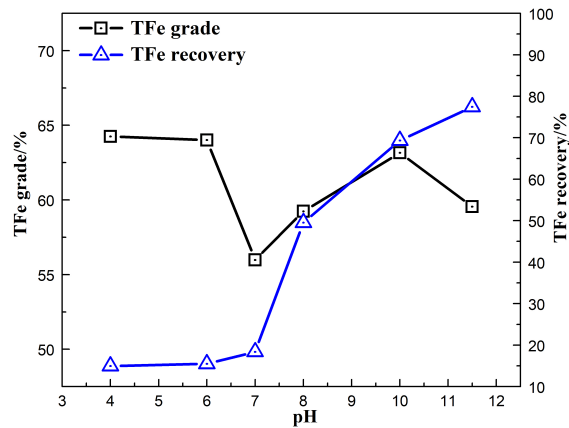
Fig. 4. The separation performances of the natural iron ores as a function of pH
