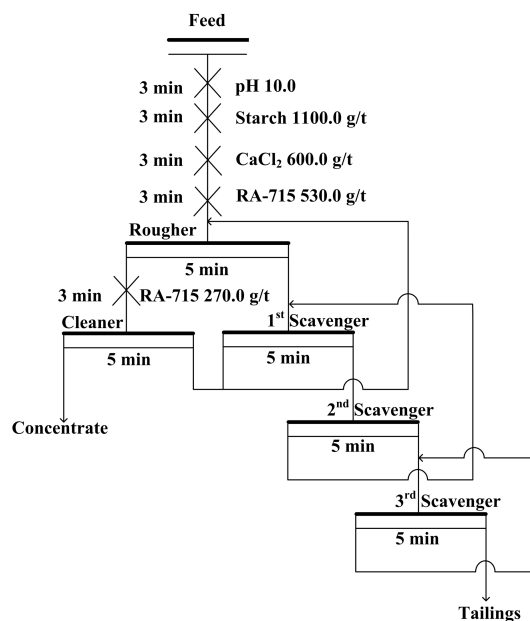
Fig. 10. The optimized flotation conditions and the flowsheet of the flotation locked cycle experiment when RA-715 was used as the collector
