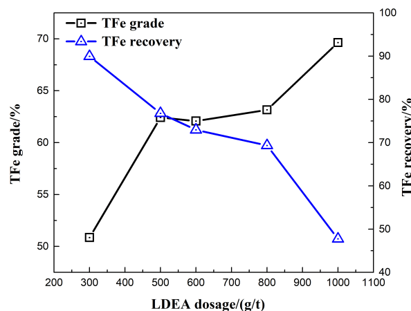
Fig. 5. The separation performances of the natural iron ores as a function of collector LDEA dosage
