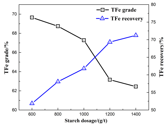
Fig. 6. The separation performances of the natural iron ores as a function of depressant starch dosage
