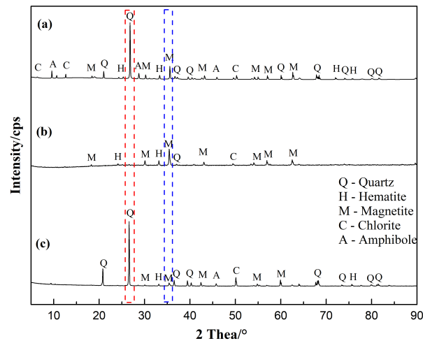
Fig. 11. XRD patterns of raw natural iron ores (a), reverse flotation concentrate (b), and tailings (c)
