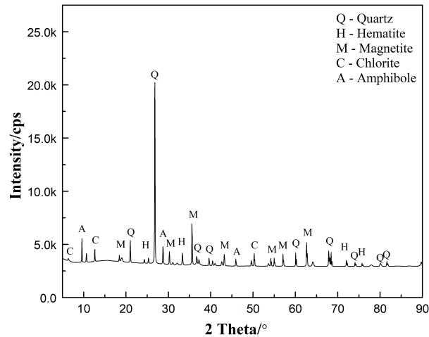
Fig. 1. X-ray diffraction patterns of the natural iron ores
