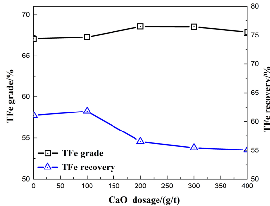
Fig. 8. The separation performances of the natural iron ores as a function of CaO dosage
