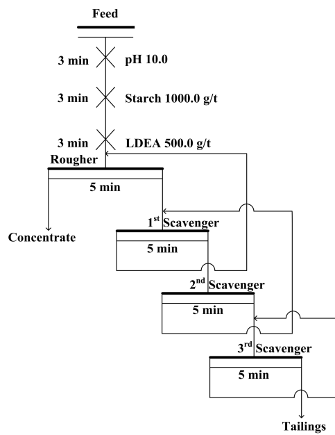
Fig. 9. The optimized flotation conditions and the flotation locked cycle experiment's flowsheet when LDEA was used as the collector
