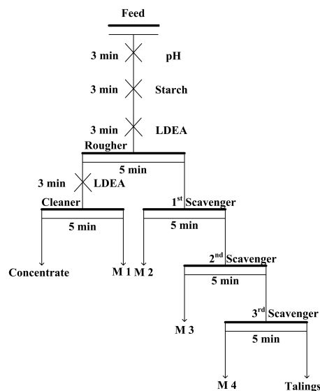
Fig. 3. The flowsheet of flotation open circuit experiment (M - middling product)
