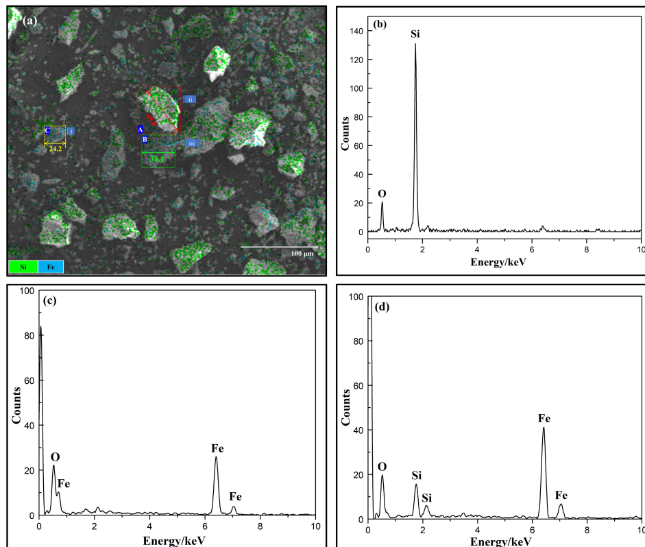
Fig. 12. SEM image and EDS analyses of the reverse flotation tailings when LDEA used as the collector (a - SEM image; b - ii point in particle A; c - i point in particle C; d - iii point in particle B)
