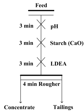
Fig. 2. The flowsheet of flotation condition experiments
