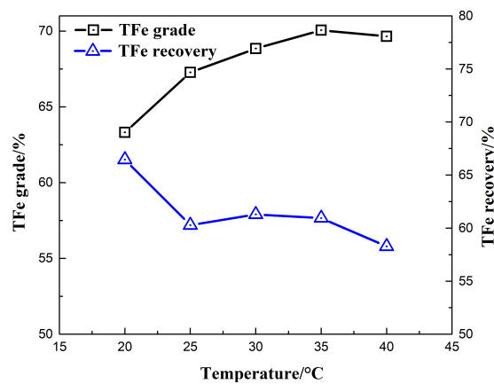
Fig. 7. The separation performances of the natural iron ores as a function of pulp temperature
