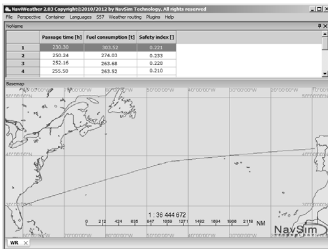
Figure 2. MEWRA prototype as a NaviWeather plugin – the final ranking of Pareto-optimal routes (Szlapczynska, 2012)
