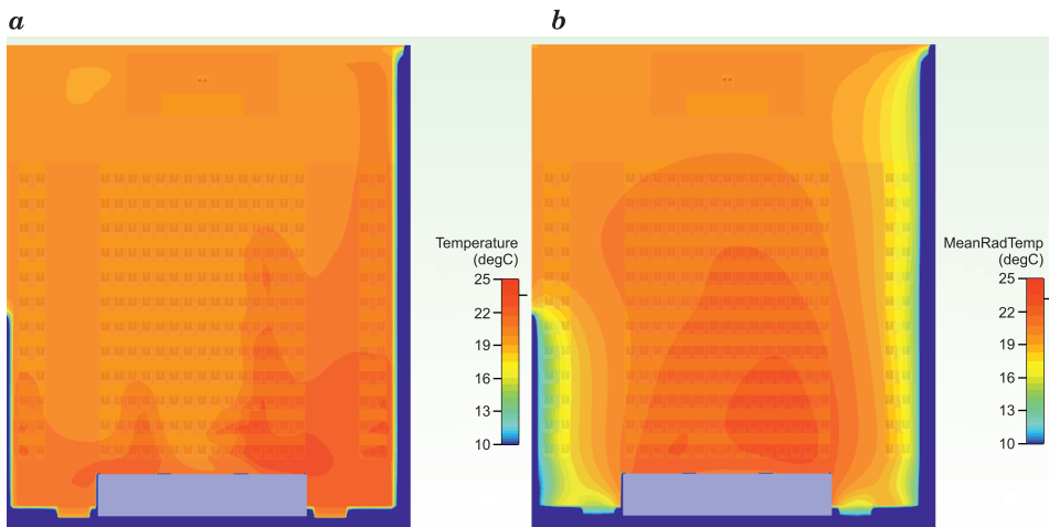
Fig. 2. The environment temperature ( a ) and the mean radiant temperature ( b ) – the results for the room filled with students in 100%, bird's eye view, distribution in a plane about 1.5 m over the floor for the highest-located seats
