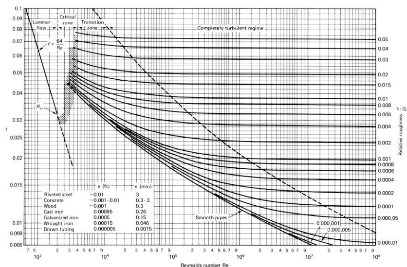
Fig. 1. Moody Diagram [4]
