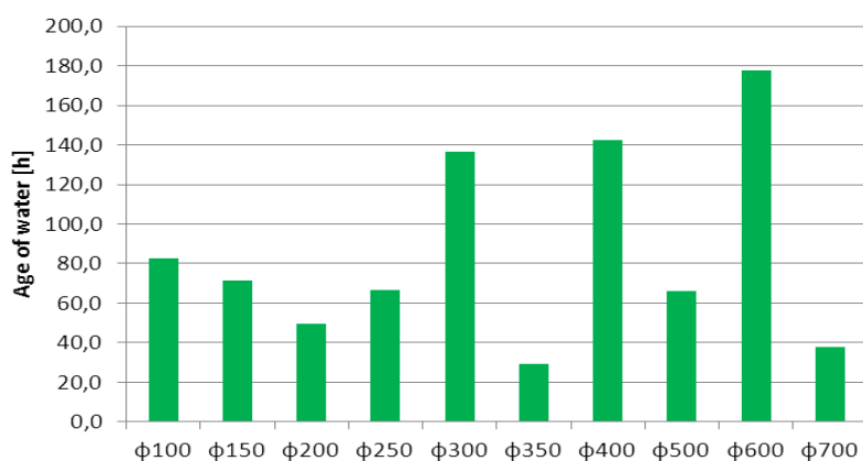
Fig. 7. Values of weighted averages of the age of water for individual pipeline diameters in Głogów
