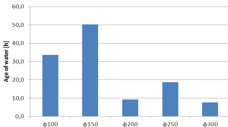
Fig. 6. Values of weighted averages of the age of water for individual pipeline diameters in Lubin
