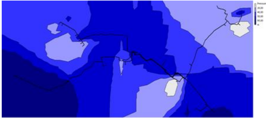
Fig. 4. Contours of water pressure levels in Lubin system during maximum water consumption
