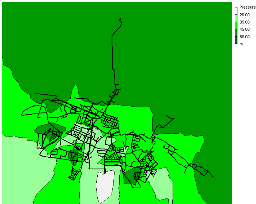
Fig. 5. Contours of water pressure levels in the Głogów system during maximum water consumption
