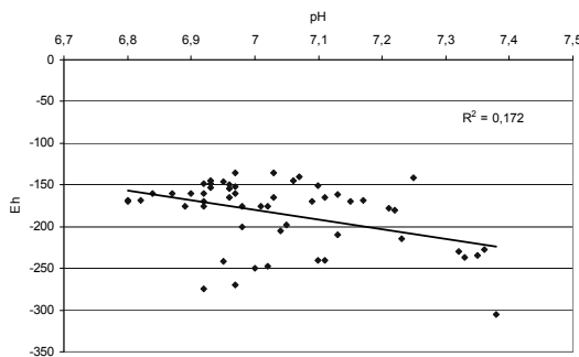
Fig. 5. Correlation between pH and Eh – Pławniowice
