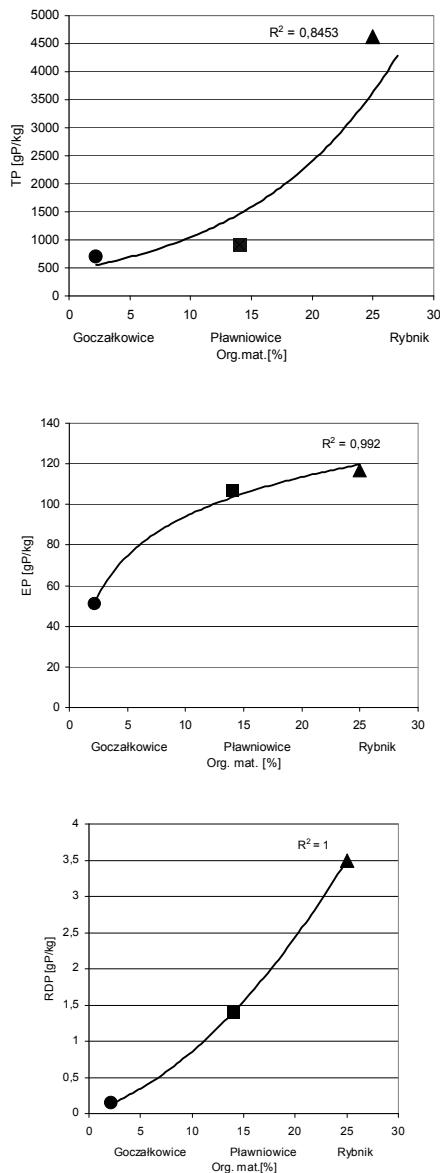
Fig. 10. Correlations between the organic matter content and concentrations of specific speciation phosphorus forms in the bottom sediments of the investigated reservoirs
