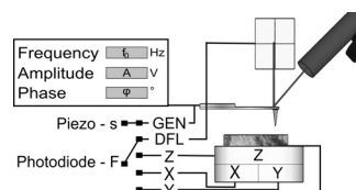
Fig. 3. Parameters of the excitation GEN and measuring response signal DFL
