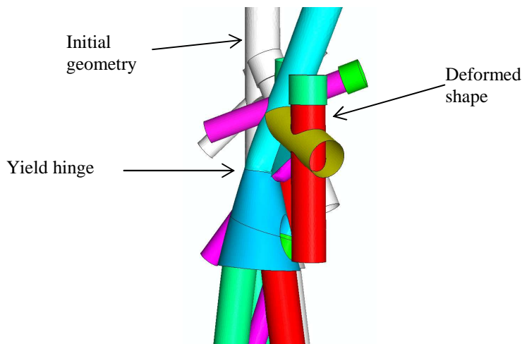
Fig. 6. The failure mechanism, scale 10:1
