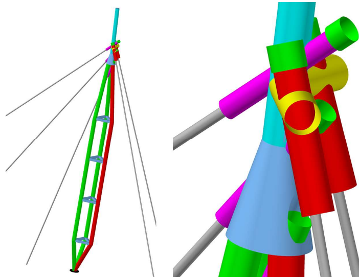
Fig. 1. Isometric view of the pylon - on the left, the steeple analyzed - on the right
