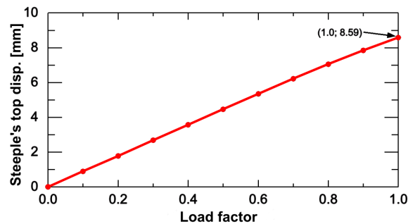
Fig. 8. Resultant displacement of the steeple's top as a function of the load factor for the strengthened structure
