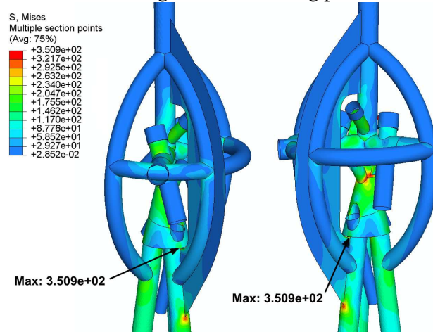
Fig. 9. Map of equivalent stresses in two different views in MPa – nonlinear analysis of the strengthened structure
