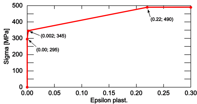
Fig. 3. The adopted stress-plastic strain relation in uniaxial stress state
