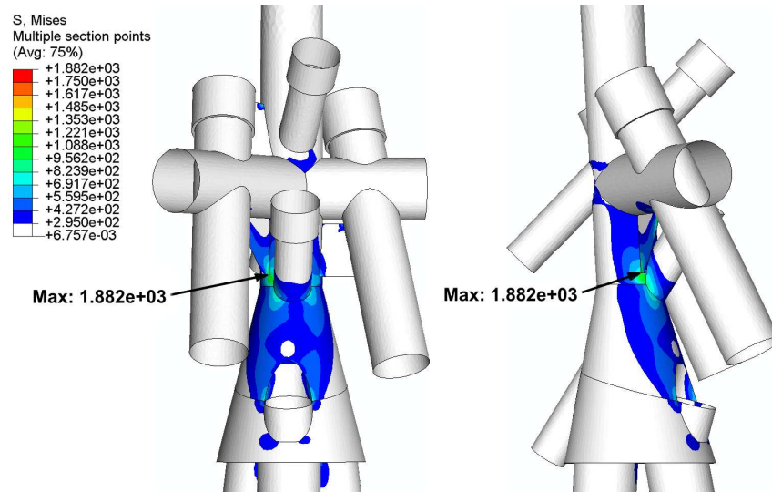
Fig. 2. Maps of equivalent stresses in two views in MPa – a linear analysis
