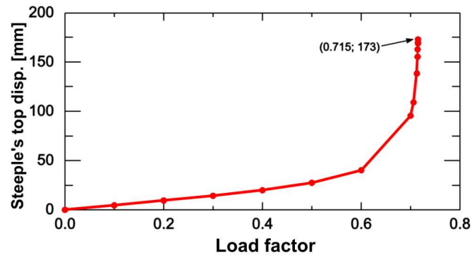
Fig. 4. Resultant displacement of the steeple's top as a function of the load factor
