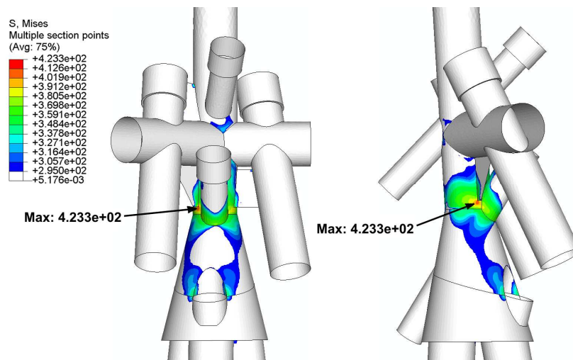
Fig. 5. Map of equivalent stresses in two different views in MPa – nonlinear analysis
