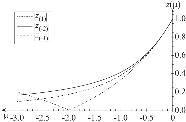
Fig. 5. Plot of the functions z_{(1)}(\mu) , z_{(-2)}(\mu) and z_{(-1/2)}(\mu) .
