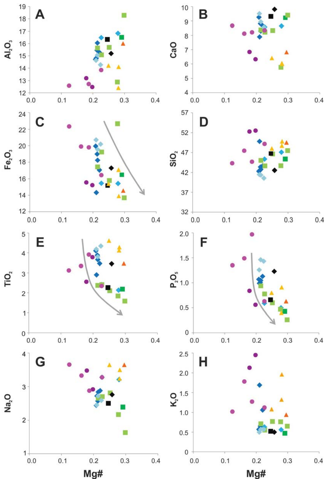
Text-fig. 8. Major element composition of Polish jotunites as a function of Mg# ( \text{MgO}/(\text{MgO} + \text{FeO}_t) ), compared to the jotunites from the Hydra Massif, the Bjerkreim-Sokndal Layered Intrusion (Rogaland Province, Norway) and Korosten Complex (Ukraine); see Table 4 for data on Polish jotunites. See Text-fig. 7 for explanation of symbols
