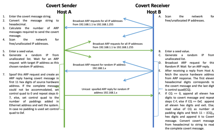
Fig. 7. Flow Diagram of ARNetSteg.
