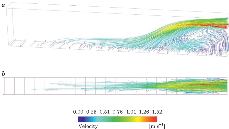
Fig. 3. Particle velocity on particle trace visualization for 300 pcs: a – side view, b – top view
