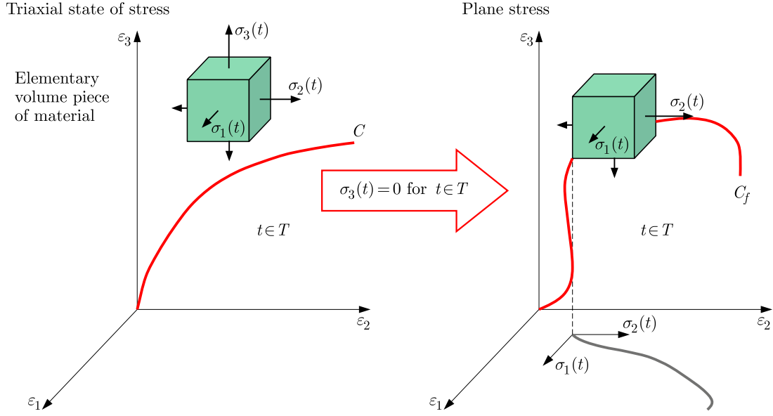
Fig. 1. Deformation paths for a triaxial and plane stress state in a material
