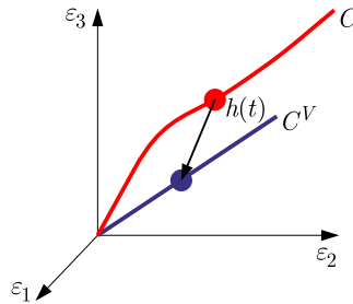
Fig. 2. Relation between the deformation path C and the path due to pure volumetric deformation C^V
