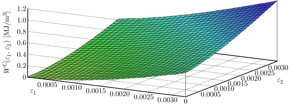
Fig. 5. The strain energy density function
