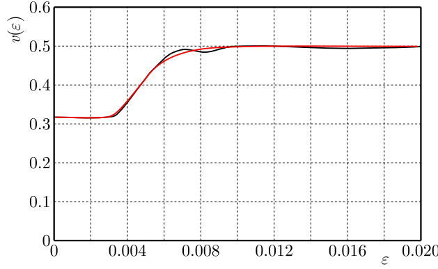
Fig. 4. Experimental plot of transversal deformation coefficient (relation between the ratio of transversal to longitudinal deformation and longitudinal deformation) and its approximation (red line)
