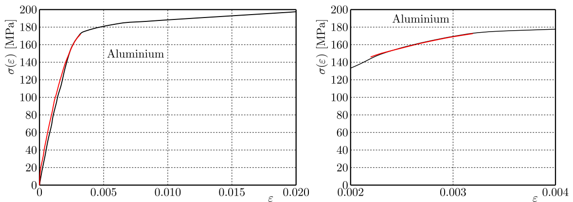
Fig. 3. Experimental relation between stress and strain (in a uniaxial tensile test) and its approximation in the nonlinear range (red line)
