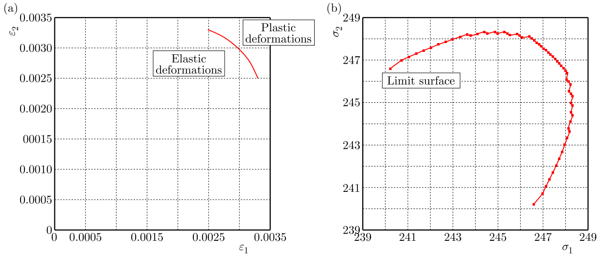
Fig. 6. Region of stability according to assumptions (4.5) in space of the deformation (a) and the stress (b) components
