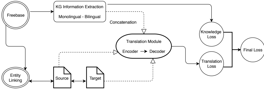
Figure 1. KG-based NMT model with monolingual and bilingual embedding constraints using entity linking system
