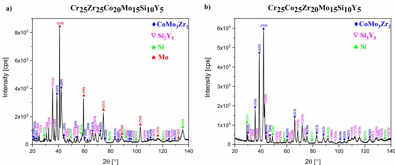
Fig. 1. Indexed X-ray diffraction patterns for a) Cr 25 Zr 25 Co 20 Mo 15 Si 10 Y 5 and b) Cr 25 Co 25 Zr 20 Mo 15 Si 10 Y 5 multicomponent alloys
