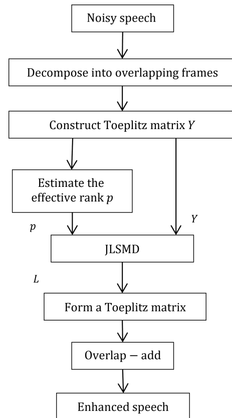
Fig. 1. Block diagram of the enhanced speech based on JLSMD for white noise.
