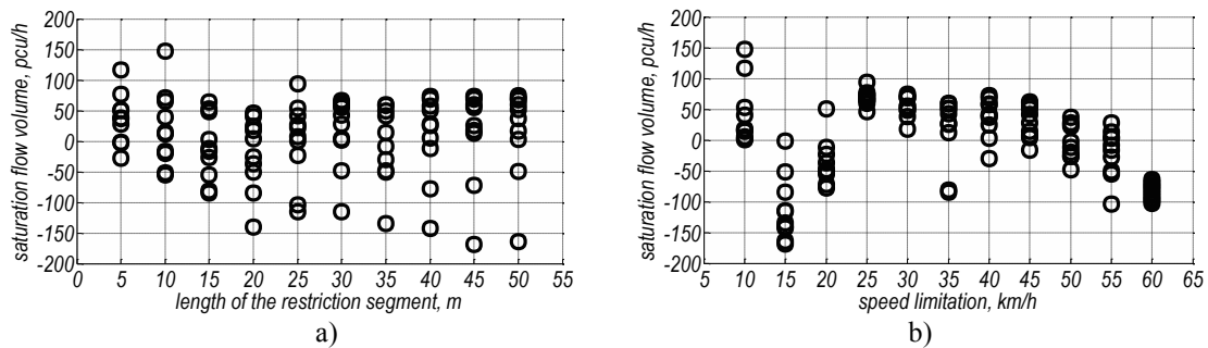
Fig. 4. Errors between experimental and theoretical data on the saturation flow volume in ‘segment length – saturation flow volume’ (a) and ‘speed limitation – saturation flow volume’ (b) coordinates
