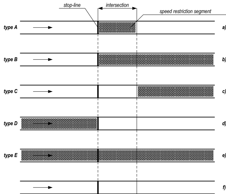
Fig. 1. Possible cases of speed limitation
