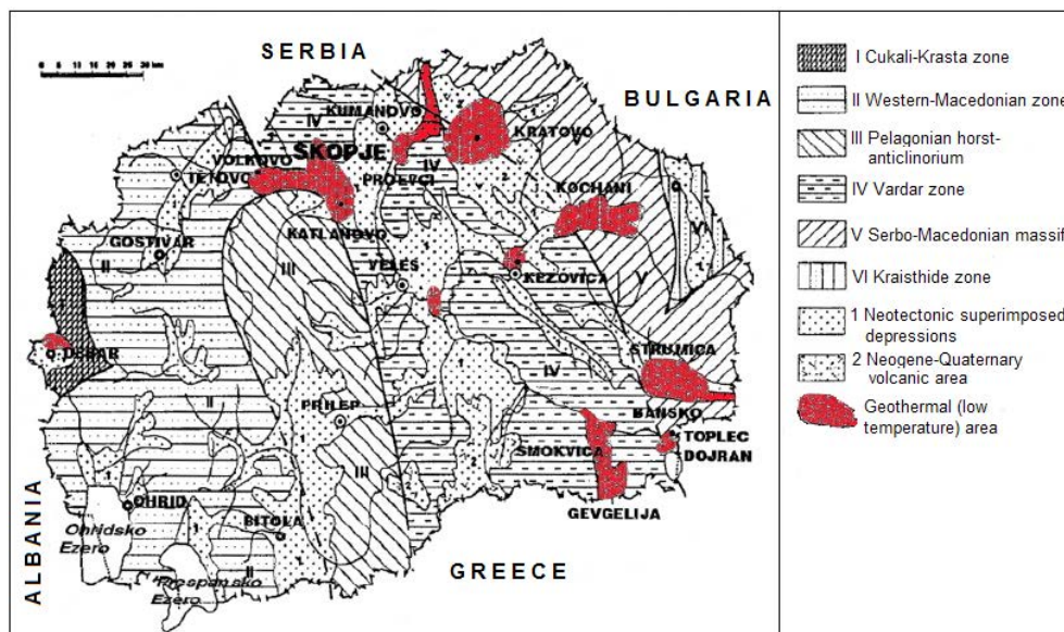
Fig. 1. Geological settings and geothermal regions in Macedonia (Arsovski 1997)
