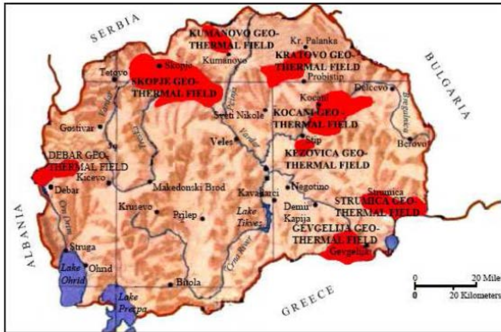
Fig. 2. Main geothermal fields in Macedonia (Popovski et al. 2005).
