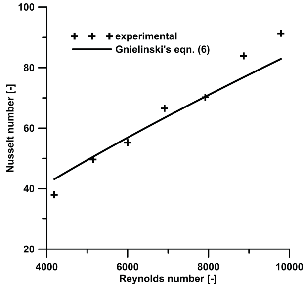
Figure 2: Comparison of experimental and calculated Nusselt number.
