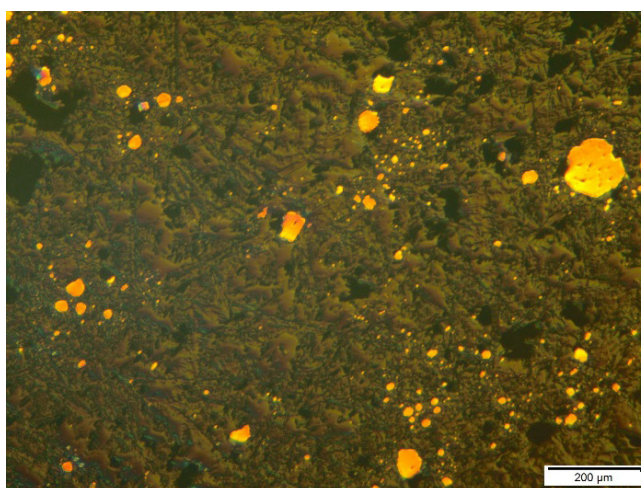
Fig. 3a. Initial coagulation of copper droplets in the liquid slag due to the CaO, and Na 2 CO 3 – chemicals addition into the suspension as in the fully industrial process
