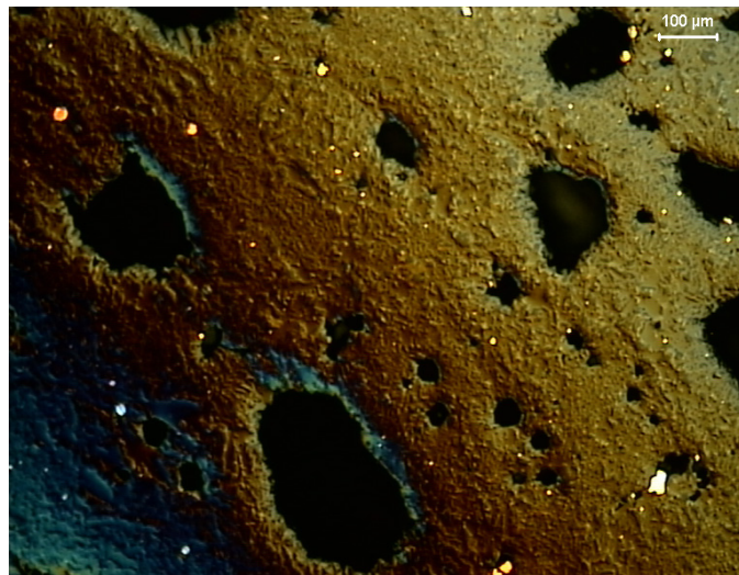
Fig. 4h. Post-processing slag containing the copper droplets; sample taken directly from the industrial process (from the smelter furnace in the Smelter and Refinery Plant, Głogów)
