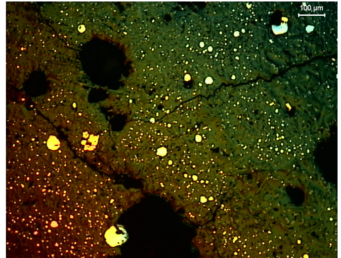
Fig. 4b. Post-processing slag containing the copper droplets; as treated by the CaO, and Na 2 CO 3 – chemicals in the conditions similar to those usually applied to the industrial practice
