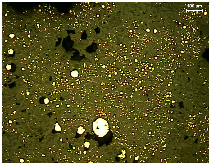
Fig. 4f. Post-processing slag containing the copper droplets; as treated by the \text{CaO} , \text{CaC}_2 , \text{NaCl} , and \text{Na}_2\text{CO}_3 – chemicals in the conditions similar to those usually applied to the industrial practice
