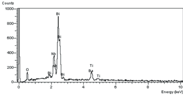
Fig. 3. The EDS analysis of 0.9BTN-0.1BBN solid solution
