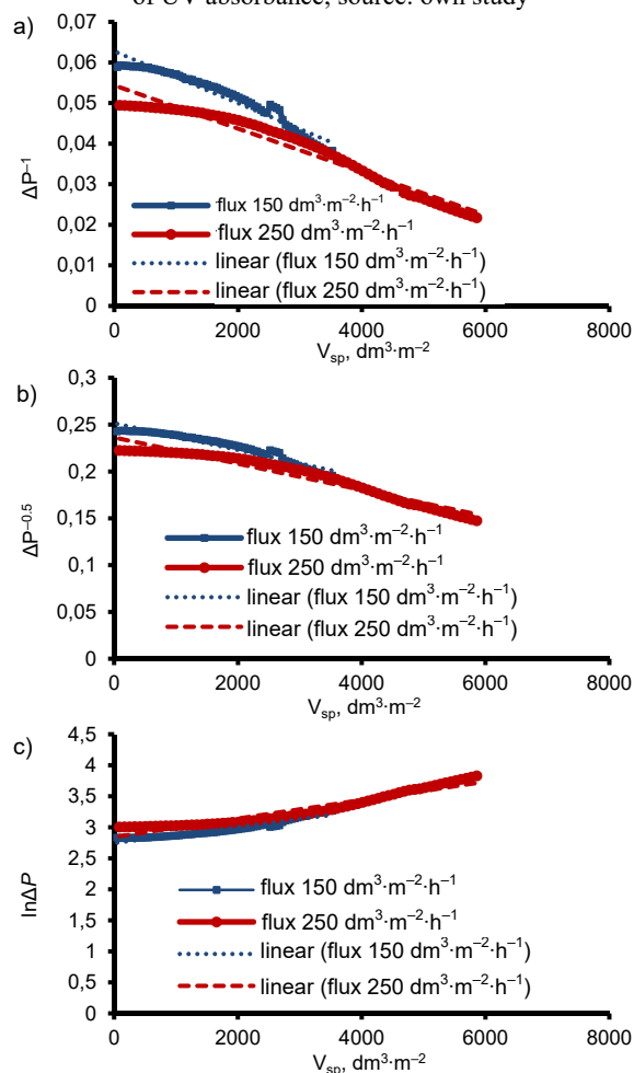
Fig. 2. Blocking filtration law analysis of \mu GAF: a) complete blocking, b) standard blocking, c) intermediate blocking law; source: own study
