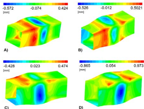
Fig. 17. Comparison of the 3D virtual geometry of the deformation zone received by numerical calculations and the experiment, A) T=1,200°C; B) T=1,300°C; C) T=1,350°C; D) T=1,400°C
