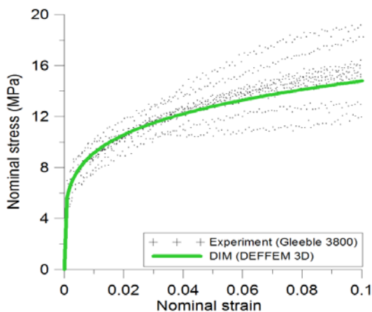
Fig. 5. Strain-stress relationships (experiment vs. calculation, T=1,300^{\circ}\text{C} , nominal strain rate =0.05\text{ s}^{-1} )
