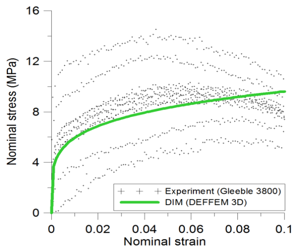
Fig. 6. Strain-stress relationships (experiment vs. calculation, T=1,450^{\circ}\text{C} , nominal strain rate =0.05\text{ s}^{-1} )
