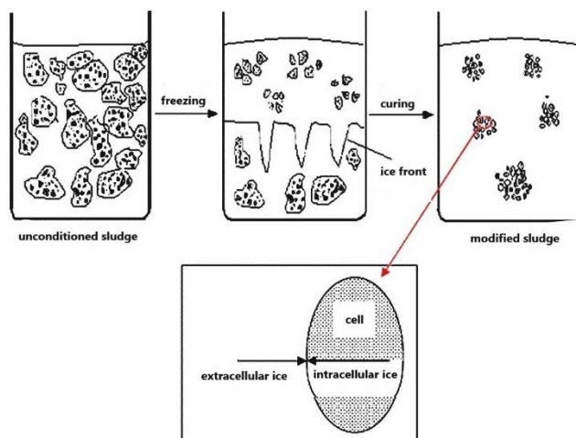
Fig. 1. The idea of freezing/thawing process of sewage sludge (Parker and Collins 1997)
