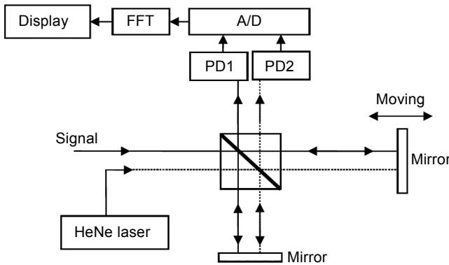
Fig. 7. Optical wavelength meter based on Michelson interferometer with HeNe calibrator laser. Two photodiodes are used to count fringes [7].
