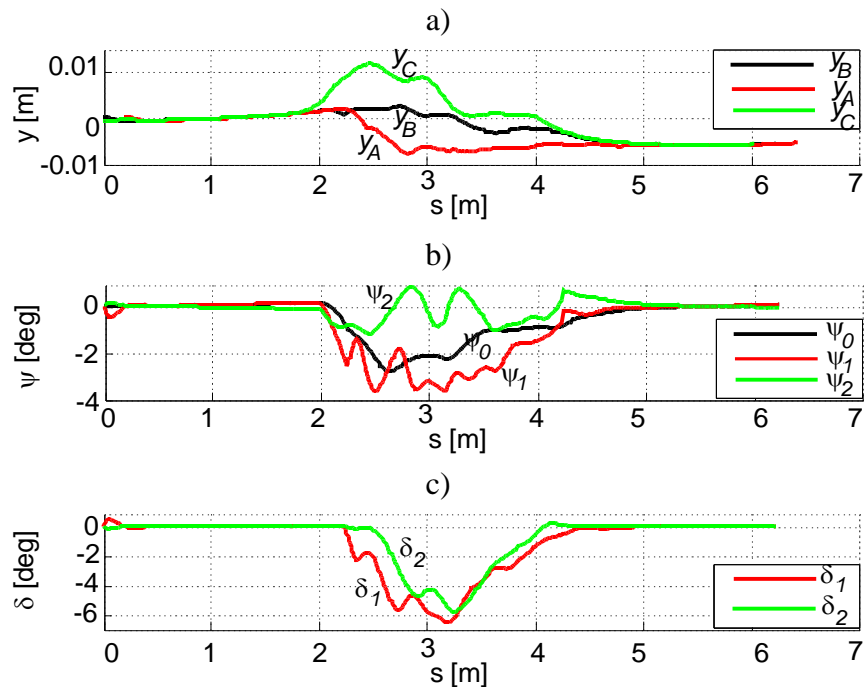
Fig. 6. Functions of the variables characterizing the way of setting vehicle axes in relation to the track centre: a) crosswise deviations y , b) angular displacements from normal \psi , c) turning angles \delta .
