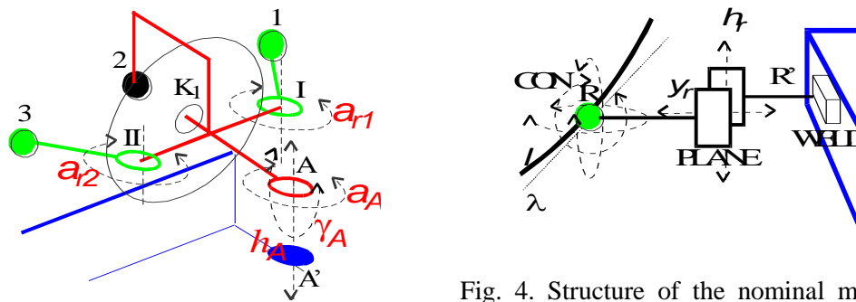
Fig. 3. Structure of the nominal model of the outer driving rollers set (close up of the front left quarter of a vehicle): Indications: h_A – distance A-A', \alpha_A , \alpha_r – rotation angles in YOX plane of the bodywork, \gamma_A – rotation angle in YOZ plane of the bodywork
