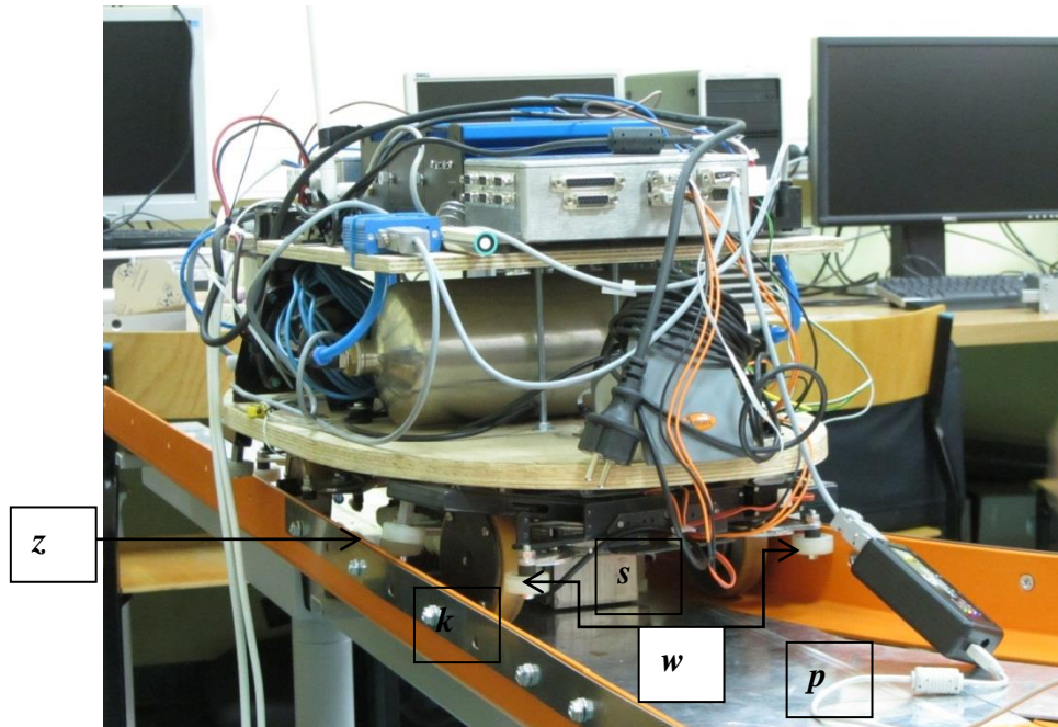
Fig. 1. State of the construction of a physical model in a \frac{1}{4} scale captured in the middle of 2012. Legend: z – outer roller, w – inner roller, k – track edge, p – track foundation, s – linear motor [4]
