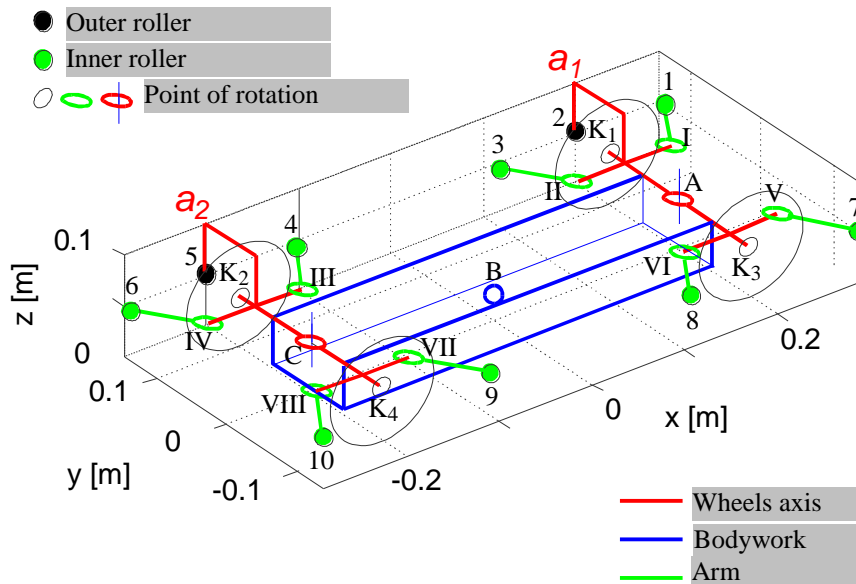
Fig. 2. Structure of dynamic model of PRT vehicle: 1 3 4 6 – left inner rollers, 7 8 9 10 – right inner rollers, 2 5 – left outer rollers, A – centre point of the front wheels axis, B – centre of bodywork, C – centre point of the rear wheels axis, I II III IV – points of rotation of the left arms, V VI VII VIII – points of rotation of the right arms, K 1 K 2 K 3 K 4 – centres of rotation of the driving wheels, \alpha_1 \alpha_2 – driving wheels axes
