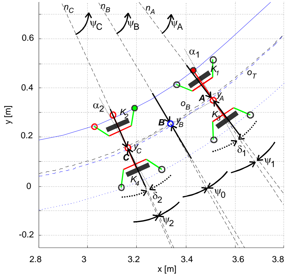
Fig. 5. State variables describing the course of motion of the model. Indications: n_A n_B n_C – normal to the track curvature (transition curve is a clothoid), y_0 y_1 y_2 distances between points of geometrical centres of rigid bodies and the track axis, \psi_0 \psi_1 \psi_2 deviations of rigid bodies axes from normal to the track curvature, \psi_A \psi_B \psi_C – intersection angles of normal, \delta_1 \delta_2 – axis turning angles
