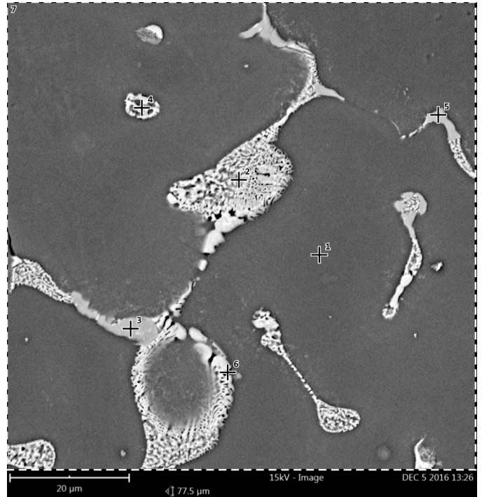
Fig. 6. Structure of the ingot cast with an average speed of 100 mm/min; cross-section (SEM)
