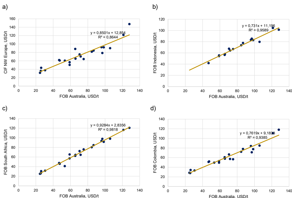
Fig. 5. Asia-Pacific market – correlation of coal index FOB Australia with coal indexes: CIF NW Europe (a), FOB Indonesia (b), FOB South Africa (c) and FOB Colombia (d)
