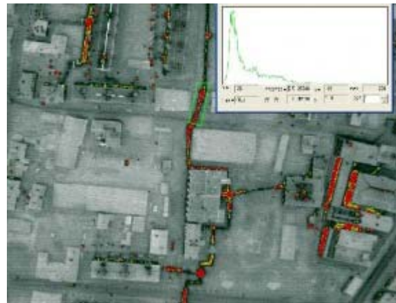
Figure 2. Aerial thermography of district heating networks [10]
