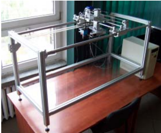
Figure 7. Experimental setup for testing vision systems [25]
