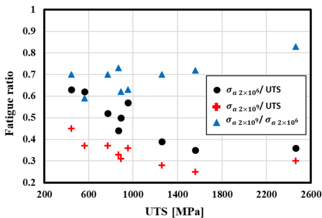
Fig. 1. Fatigue results \sigma_{a2 \times 10^6} (●), \sigma_{a2 \times 10^9} (+), \sigma_{a2 \times 10^9}/\sigma_{a2 \times 10^6} (▲) vs. UTS of tested structural steels
