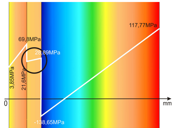
Fig. 5. Hoop stress distribution for the numerical model covered with a 300 μm thick layer of La 2 Zr 2 O 7 and the thickness of interlayer 250 μm
