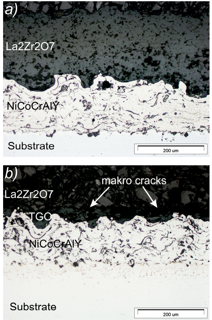
Fig. 7. The thermal barrier coating with La_2Zr_2O_7 insulation layer: a) initial state of destruction process; b) effect of crack growth in the TGO sublayer to form of macro-cracks in the top ceramic surface after 48 h exposure
