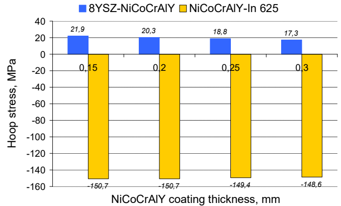
Fig. 4. Graph of hoop stress distribution in the model coated with a 300 μm thick 8YSZ layer on the NiCoCrAlY bond-coat and on the In 625 substrate material for different bond coat thicknesses
