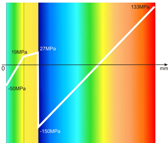
Fig. 3. Hoop stress distribution for the numerical model covered with a 300 μm thick layer of 8YSZ and the thickness of interlayer 250 μm
