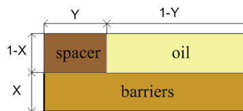
Fig. 1. Geometric arrangement of insulation system ( XY model)
