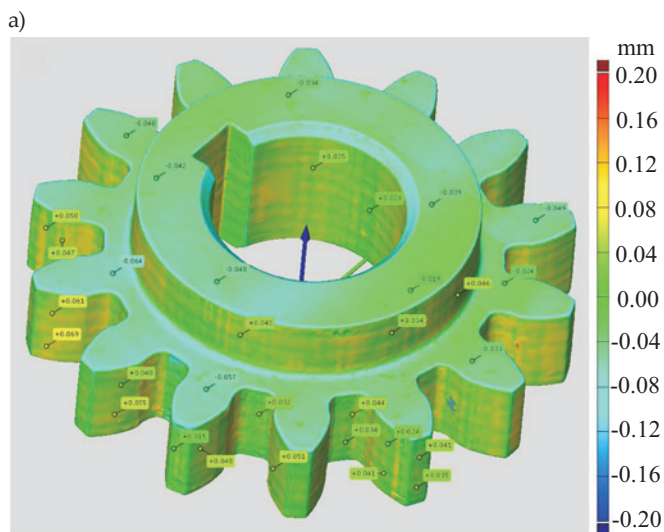
Fig. 2. Dimensional deviations of: a) gear made from FullCure720 RGD720 material, b) the profile of gear
