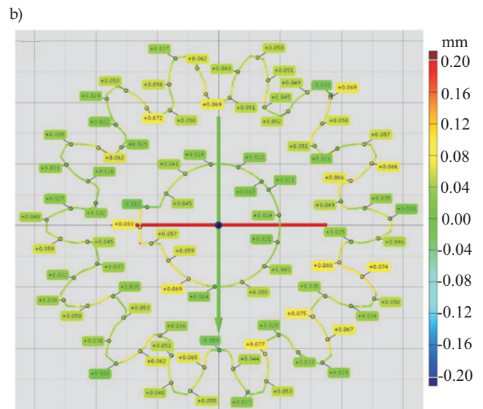
Fig. 2. Dimensional deviations of: a) gear made from FullCure720 RGD720 material, b) the profile of gear
