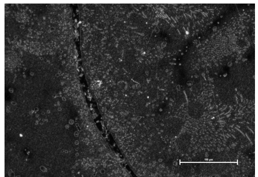
Fig. 3. The microstructures of archaeological material from Chelmiec (site 21) marked CH01a. The visible structure of copper with its oxygen eutectic \text{Cu}_2\text{O} and metallic contamination. The image in the bright (a) and dark field (b). Magnification of 200x
