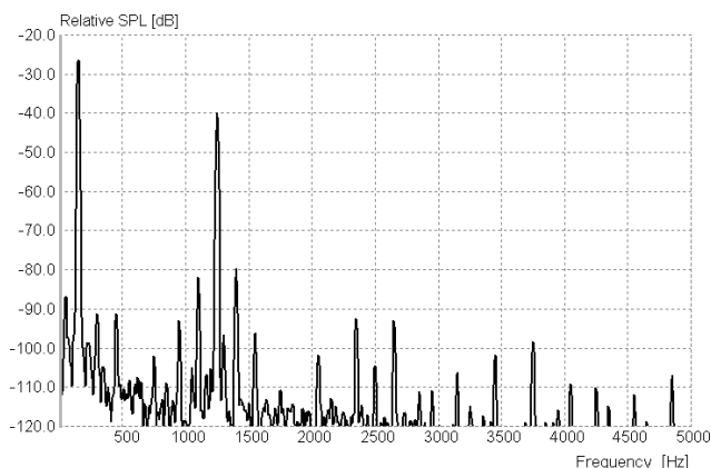
Fig. 7. Mid-woofer #1 modulation distortion: 150/1250 Hz, CC.
