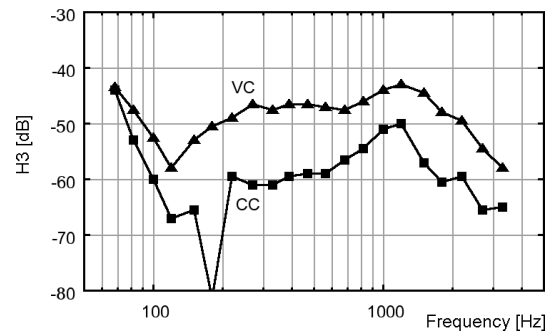
Fig. 10. Mid-woofer #2 3rd harmonic distortion; level 2.83 Vrms.
