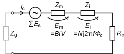
Fig. 1. Electrical equivalent circuit for a speaker driver.
