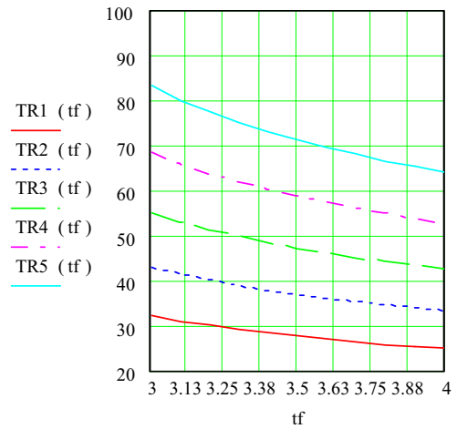
Fig. 10. Temperatures TR [°C] in case of cooling according to time t_f [s]
