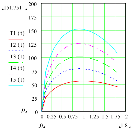
Fig. 5. Variation of temperatures T [ ^\circ C ] according to time t [s]
