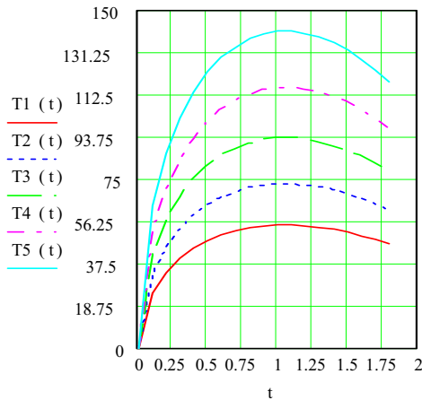
Fig. 7. Variation of temperatures T [ ^\circ\text{C} ] according to time t [s]
