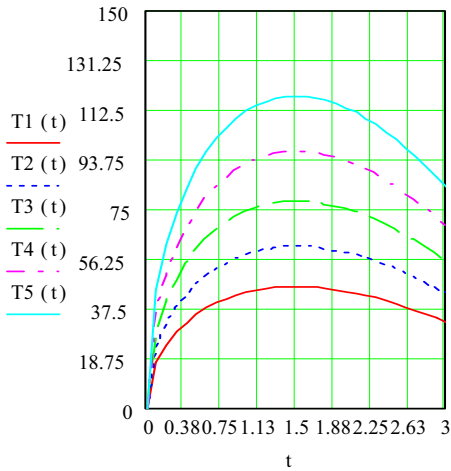
Fig. 9. Variation of temperatures T [°C] according to time t [s]
