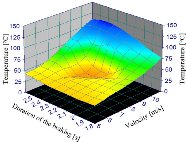
Fig. 2. Temperature variation at the friction surface for the emergency braking
