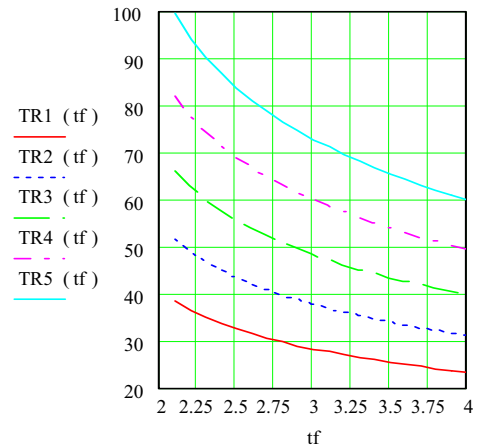
Fig. 8. Temperatures TR [ ^\circ\text{C} ] in case of cooling according to time t_f [s]
