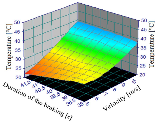
Fig. 3. Temperature variation at the friction surface for the service braking
