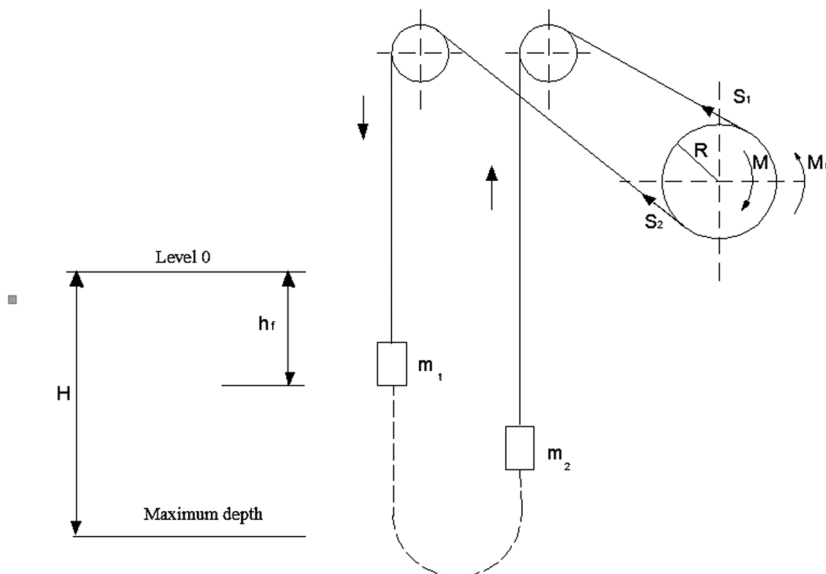
Fig. 4. Hoisting installation. Diagram for the determination of the spreader energy in the braking process
