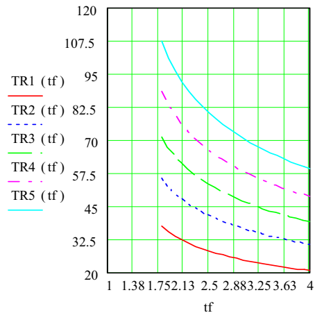
Fig. 6. Temperatures TR [ ^\circ C ] in case of cooling according to time t_f [s]
