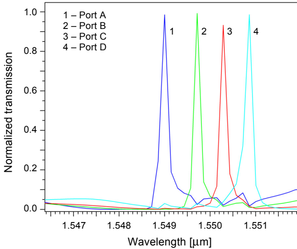
Fig. 3. Output spectrums in ports A, B, C and D.
