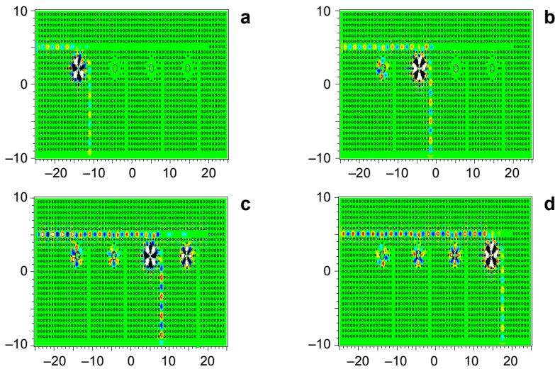
Fig. 4. The calculated field distribution inside the structure at four wavelengths: 1549 (a), 1549.7 (b), 1550.3 (c) and 1550.9 nm (d).
