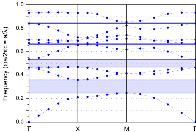
Fig. 1. The band structure diagram of the proposed PhC.
