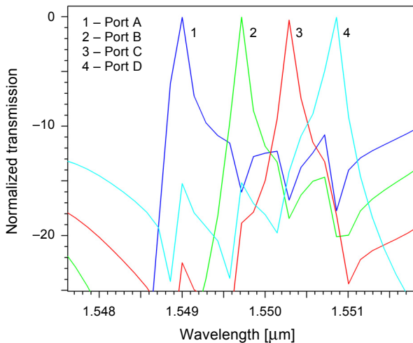
Fig. 5. Output spectrums in ports A, B, C and D in decibel scale.
