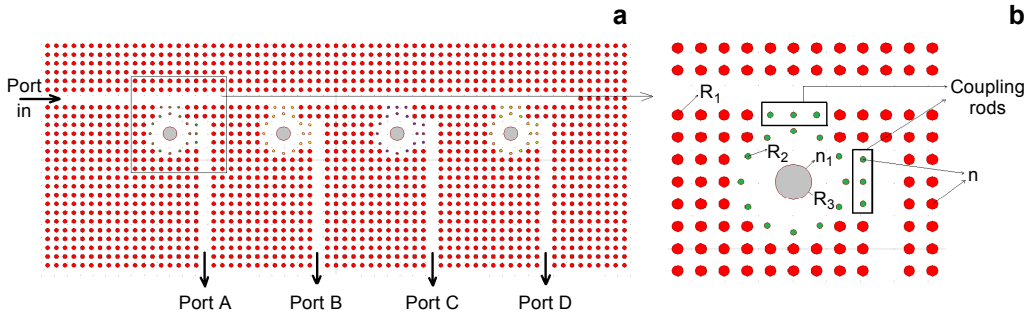
Fig. 2. The schematic diagram of the proposed demultiplexer (a); a macroscopic view of the first resonant ring (b).
