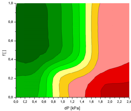
Fig. 5. An “area of risk” determined on the basis of membership functions and the set of rules from the discussed example
