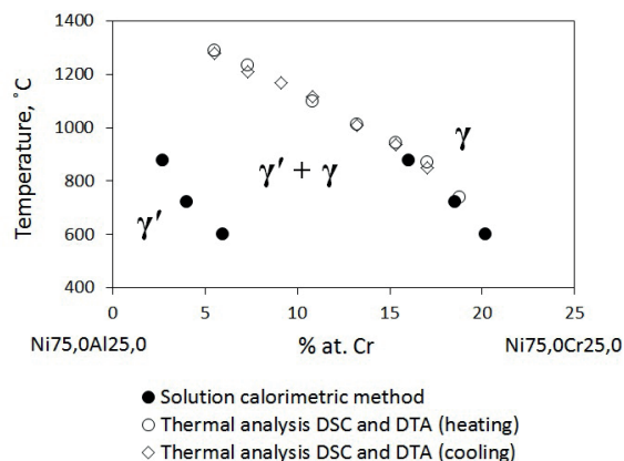
Fig. 12 Compilation of phase boundaries \gamma' / \gamma'+\gamma and \gamma'+\gamma / \gamma obtained in this paper and with use of solution calorimetric method [12].
