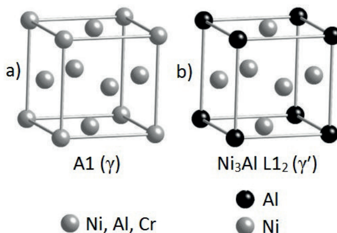
Fig. 1 Elementary cell a) disordered phase \gamma in Ni–Al–Cr system; b) ordered phase \gamma' (intermetallic phase Ni 3 Al)
