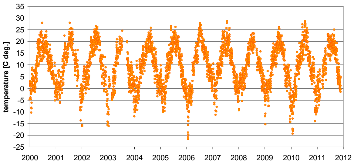
Fig. 2. Daily temperature averages at JOZE during 12 years (local sensor)
