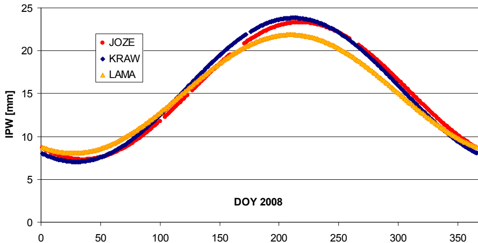
Fig. 8. Integrated precipitable water annual model for 3 EPN stations in Poland (EPN combined tropospheric product) 2008
