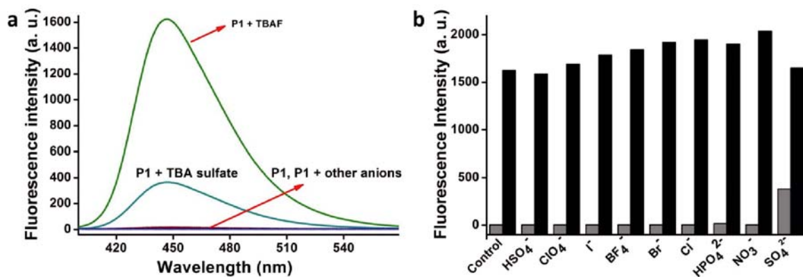
Figure 2. a) Fluorescence spectra of P1 (10 \mu\text{M} ) toward various anions (50 \mu\text{M} ) in acetonitrile with incubation of 1 min, \lambda_{\text{ex}} = 387 nm. b) Fluorescence intensity response of P1 (10 \mu\text{M} ) with various analytes in acetonitrile, \lambda_{\text{ex}} = 387 nm. grey bar: probe + analytes (50 \mu\text{M} ); Black bar: probe + \text{F}^- (50 \mu\text{M} ) + analytes (50 \mu\text{M} )
