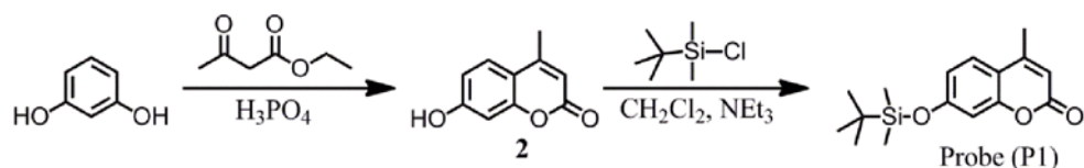
Scheme 1. Synthesis of probe (P1)
