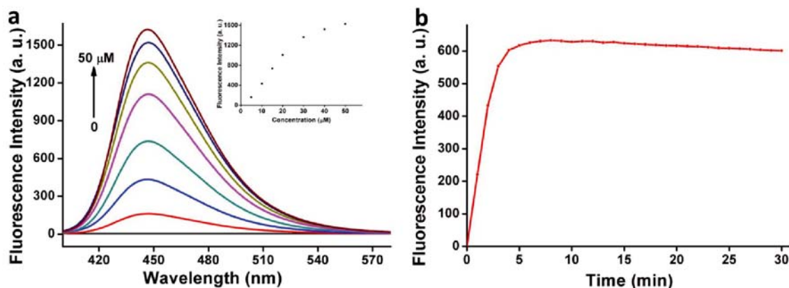
Figure 3. a) Fluoride concentration-dependent fluorescence intensity change of P1 in acetonitrile. b) Time-dependent fluorescence intensity change of P1 (10 μM) with 10 μM TBAF, \lambda_{\text{ex}} = 387 nm
